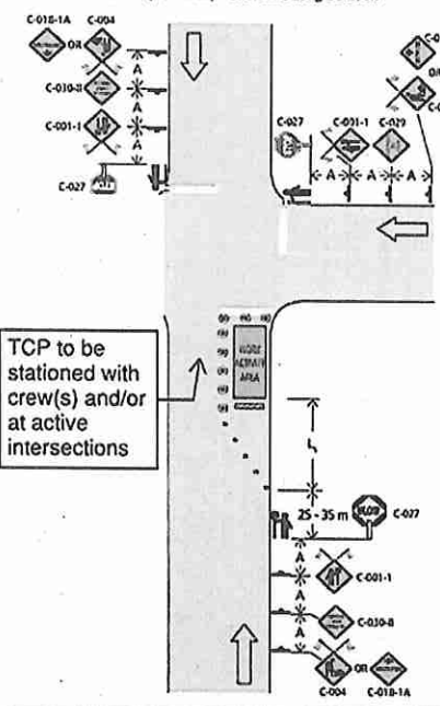
Figure 11.2: Intersection Lane Closure – Two-Lane, Two-Way Roadway with TCPs (Near Side) – Short and Long Duration
