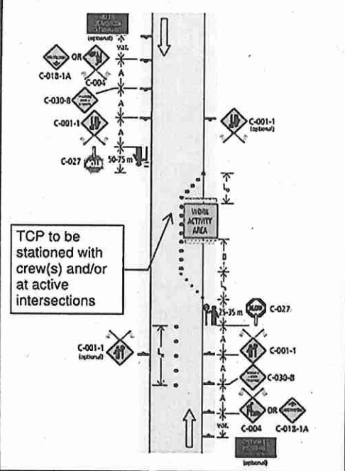
Figure 7.6: Lane Closure with TCPs – Single Lane Alternating – Short and Long Duration
